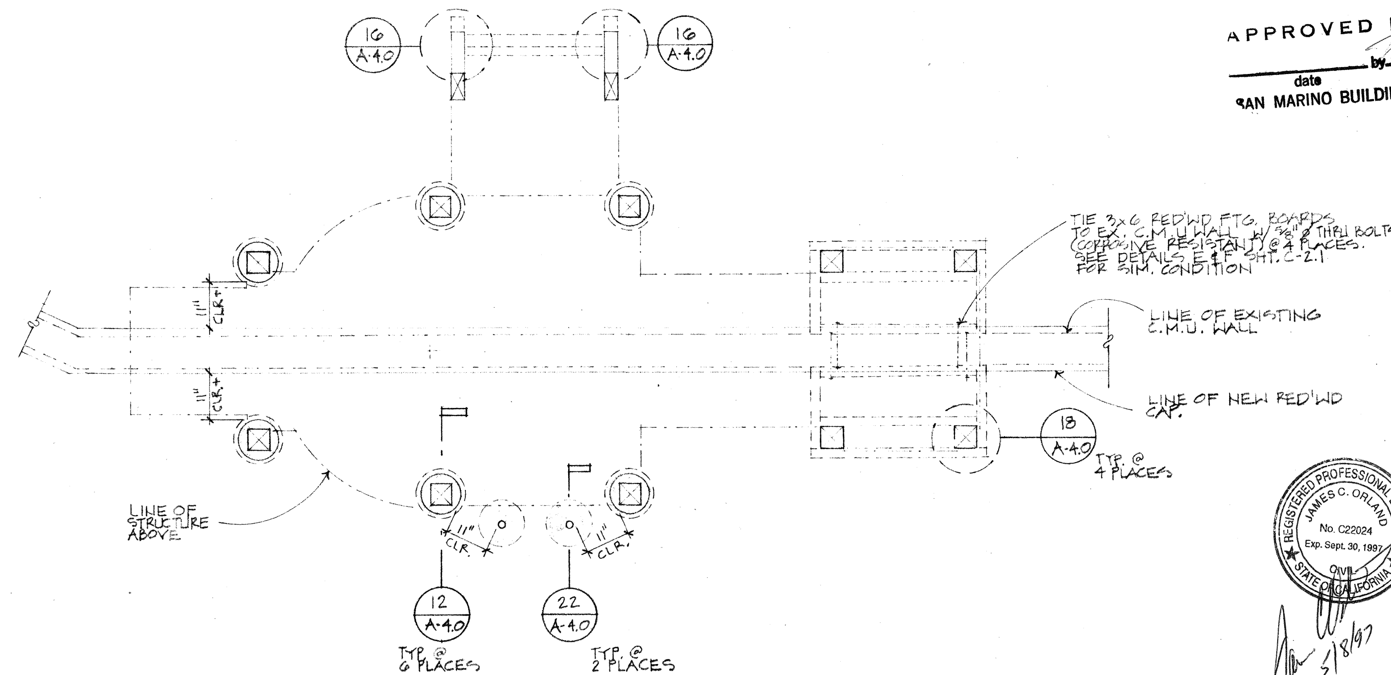
Foundation Plan
